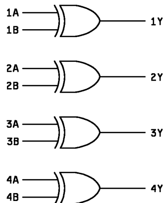
FIGURE 3. Logic diagram.
