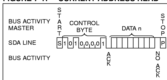
FIGURE 7-1: CURRENT ADDRESS READ
