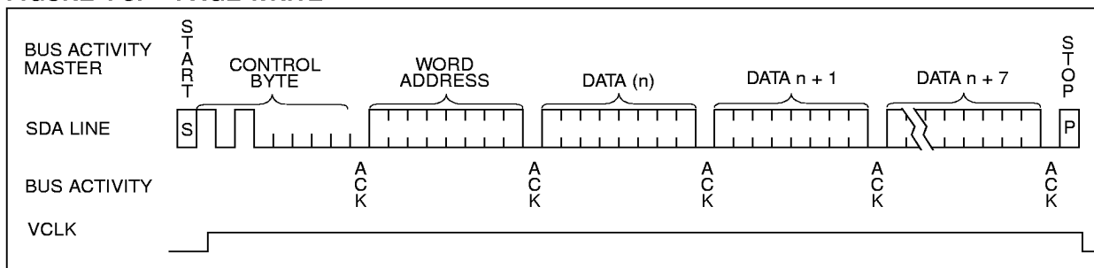
FIGURE 4-3: PAGE WRITE
