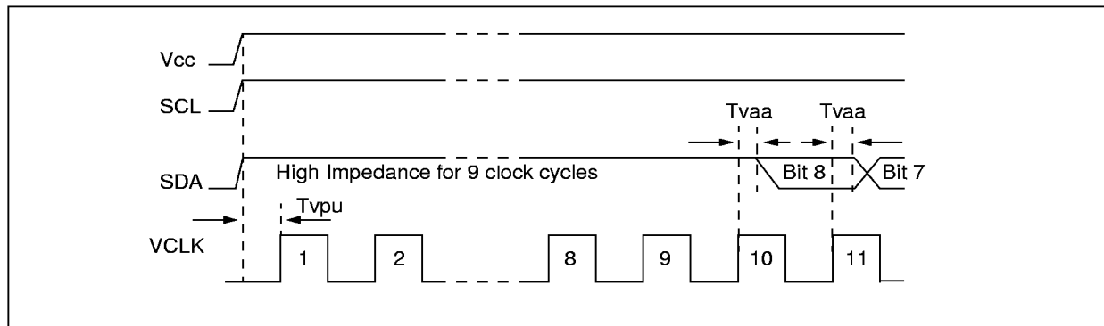
FIGURE 2-2: DEVICE INITIALIZATION
