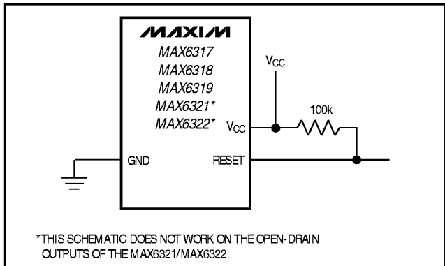
Figure 9. Ensuring \overline{\text{RESET}} Valid to V_{CC} = 0 on Active-High Push/Pull Outputs
