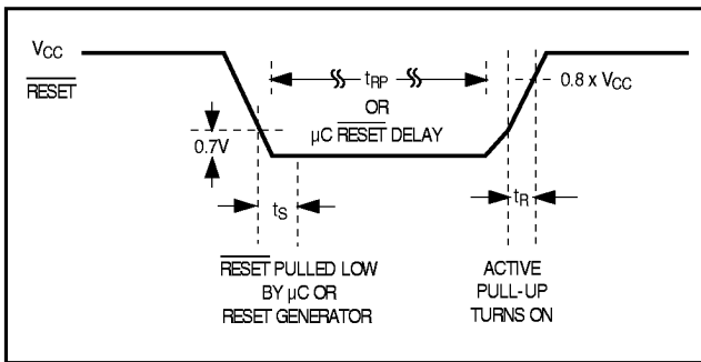
Figure 5. Bidirectional \overline{\text{RESET}} Timing Diagram
