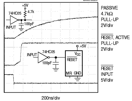
MAX6316M/6318MH/6319MH BIDIRECTIONAL PULL-UP CHARACTERISTICS
