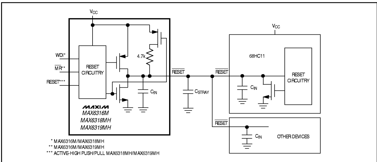
Figure 3. MAX6316M/MAX6318MH/MAX6319MH Supports Additional Devices on the Reset Bus
