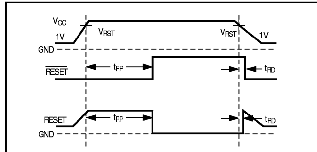
Figure 2. Reset Timing Diagram
