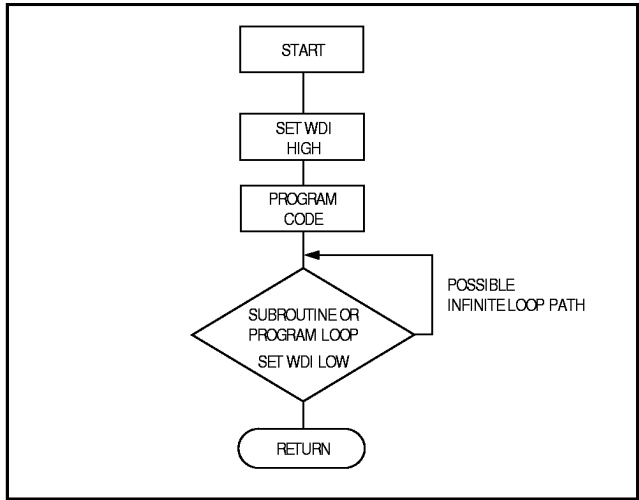
Figure 10. Watchdog Flow Diagram
