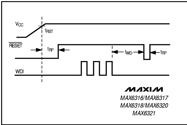
Figure 7. Watchdog Timing Relationship
