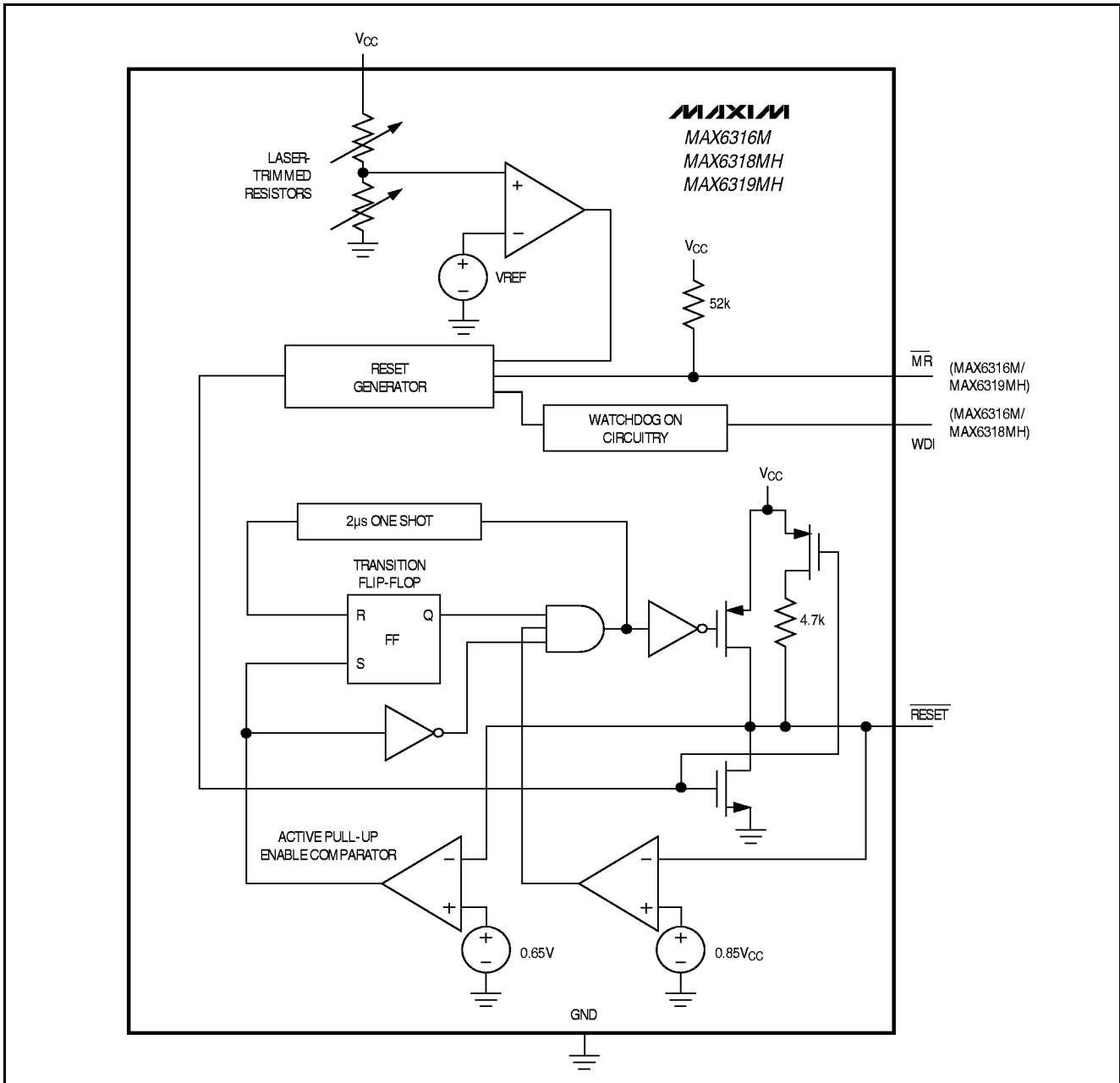
Figure 4. MAX6316/MAX6318MH/MAX6319MH Bidirectional Reset Output Functional Diagram
