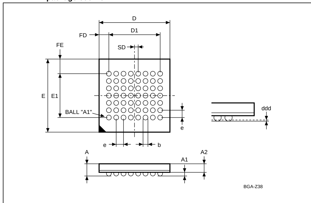
Figure 18. VFBGA56 7.7 × 9mm - 8×7 active ball array, 0.75mm pitch, bottom view package outline
