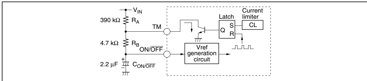
Figure 6.1 Connection Diagram (example)
