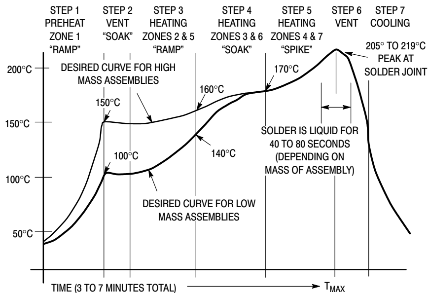
Figure 2. Typical Solder Heating Profile
