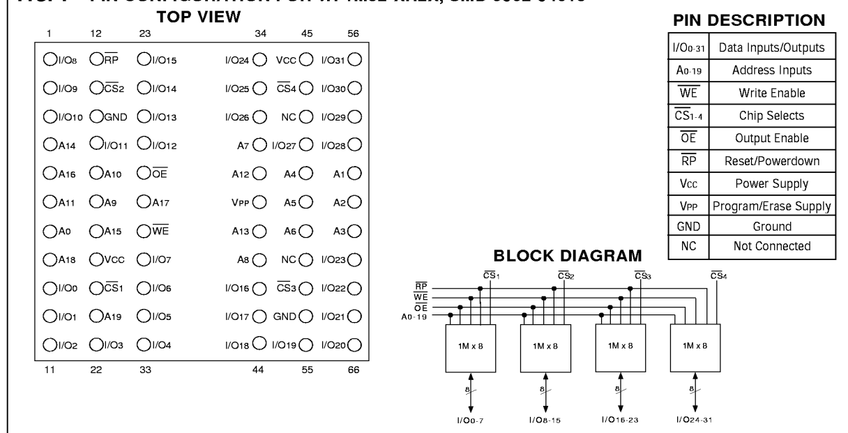
FIG. 1 PIN CONFIGURATION FOR WF1M32-XH2X, SMD 5962-94613
