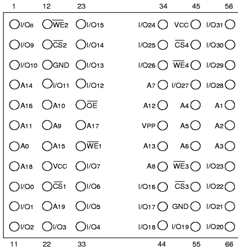
FIG. 10 PIN CONFIGURATION FOR WF1M32E-XH2X
