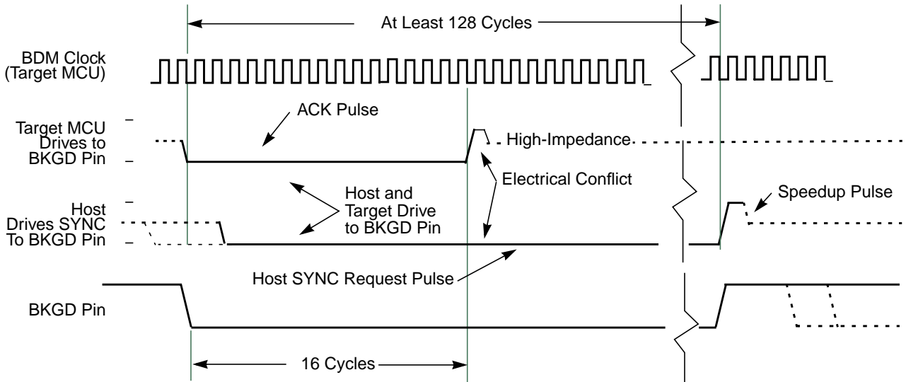
Figure 15-14. ACK Pulse and SYNC Request Conflict
