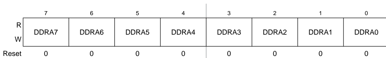
Figure 24-5. Port A Data Direction Register (DDRA)
