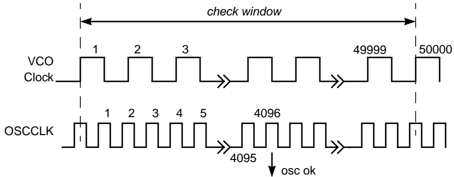
Figure 2-19. Check Window Example
