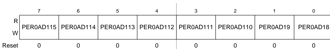
Figure 24-66. Port AD1 Pull Up Enable Register 0 (PER0AD1)
