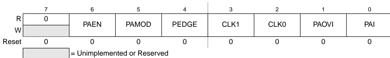
Figure 7-35. 16-Bit Pulse Accumulator Control Register (PACTL)
