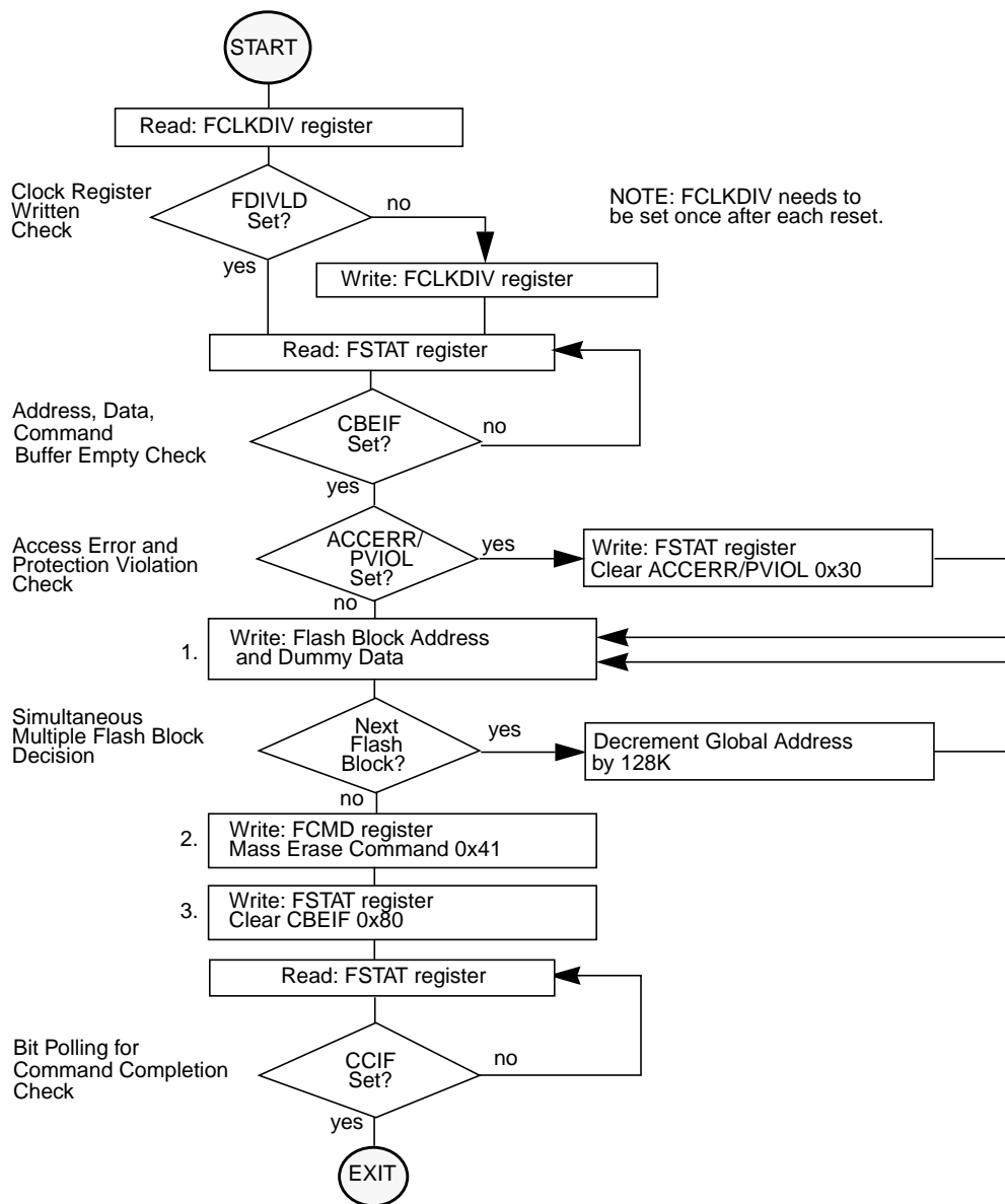
Figure 27-30. Example Mass Erase Command Flow
