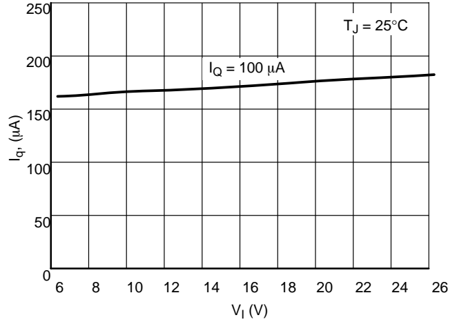
Figure 17. Current Consumption I_q vs. Input Voltage V_1
