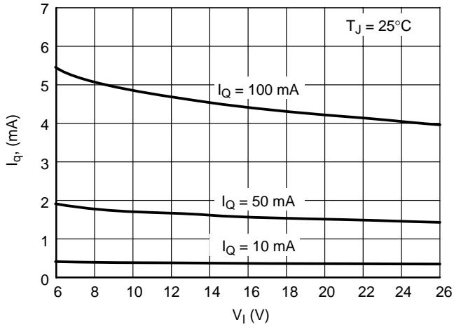
Figure 16. Current Consumption I_q vs. Input Voltage V_1
