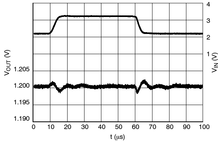
Figure 27. Line Transients, 1.2 V Version, t_R = t_F = 5 \mu\text{s} , I_{OUT} = 30 \text{ mA}
