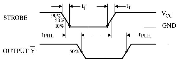
Figure 5. Switching Waveforms
