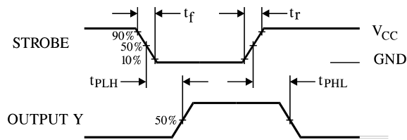
Figure 4. Switching Waveforms
