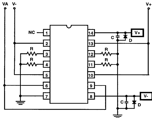
STATIC CONFIGURATION HS-302RH/303RH/306RH/307RH/883S
