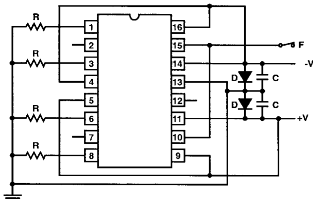
DYNAMIC CONFIGURATION HS-384RH/390RH/883S
