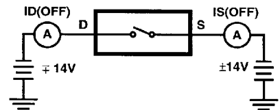
FIGURE 5. OFF LEAKAGE CURRENT TEST CIRCUIT (I S(OFF) , I D(OFF) )
