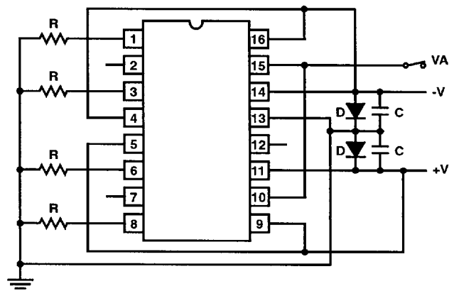
STATIC CONFIGURATION HS-384RH/390RH/883S
