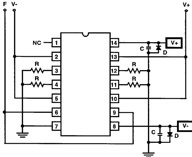
DYNAMIC CONFIGURATION HS-306RH/307RH/883S
