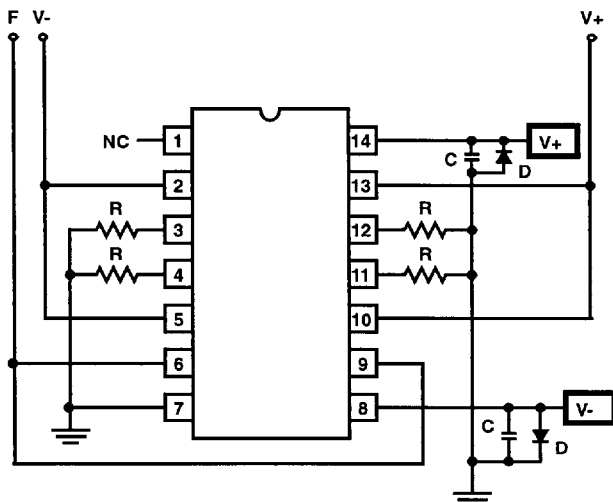
DYNAMIC CONFIGURATION HS-302RH/303RH/883S
