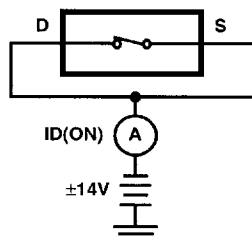
FIGURE 4. ON LEAKAGE CURRENT TEST CIRCUIT (I D(ON) )
