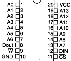
Pinout DIL 20 pins (top view)
