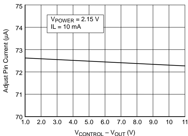
Figure 13. Adjust Pin Current vs V_{\text{CONTROL}} - V_{\text{OUT}}
