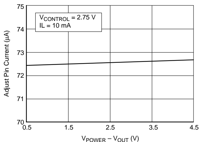
Figure 14. Adjust Pin Current vs V_{\text{POWER}} - V_{\text{OUT}}
