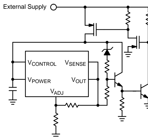
Figure 17. Example Clamp Circuitry for V_{POWER} - V_{OUT} > 6.0 \text{ V}
