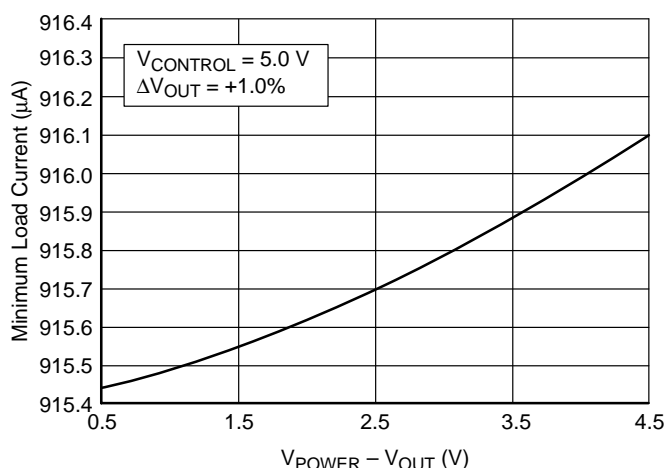
Figure 15. Minimum Load Current vs V_{\text{POWER}} - V_{\text{OUT}}
