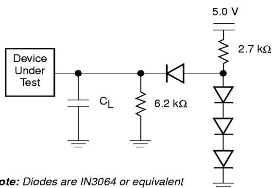
Figure 6. Test Setup
