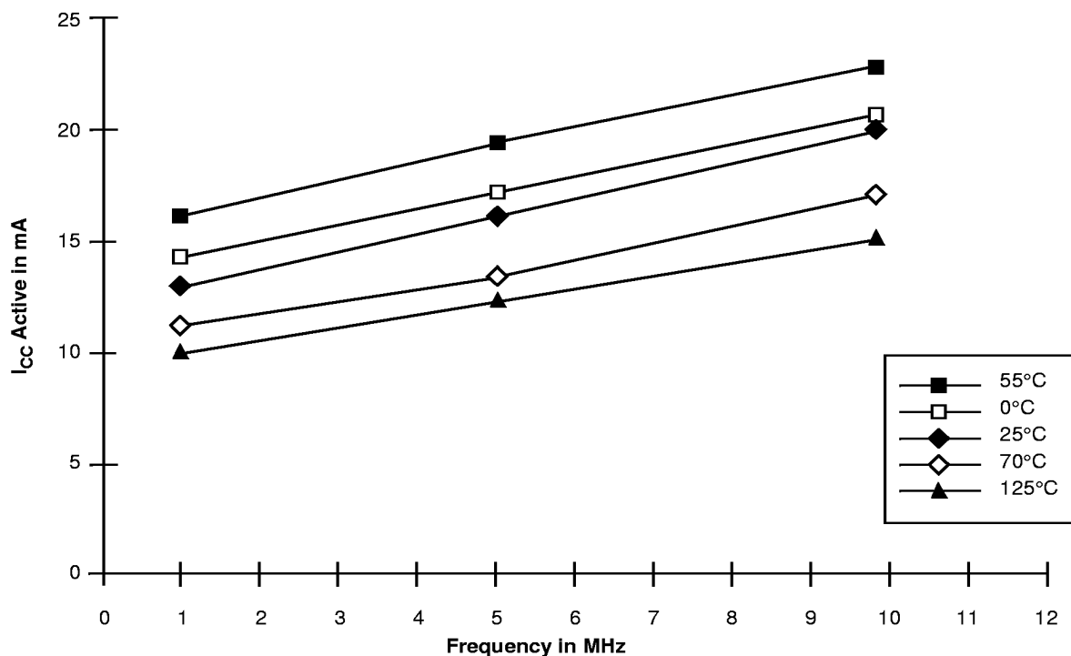
Figure 5. Am28F512—Average I_{CC} Active vs. Frequency
