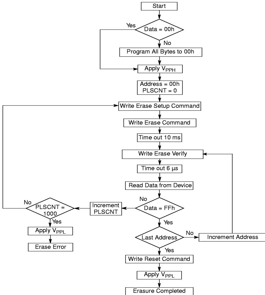
Figure 1. Flasher Electrical Erase Algorithm
