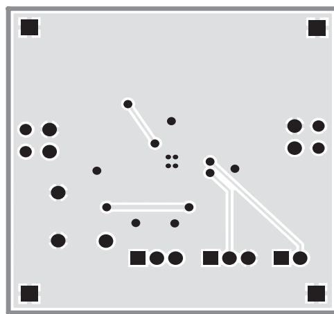
Figure 7: AAT2556 Evaluation Board Bottom Side Layout.
