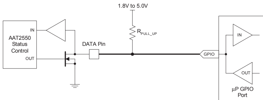
Figure 3: Data Pin Application Circuit.
