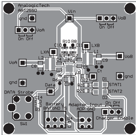
Figure 5: AAT2550 Evaluation Board Top Side Layout.
