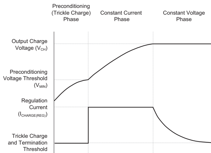
Figure 1: Typical Charge Profile.
