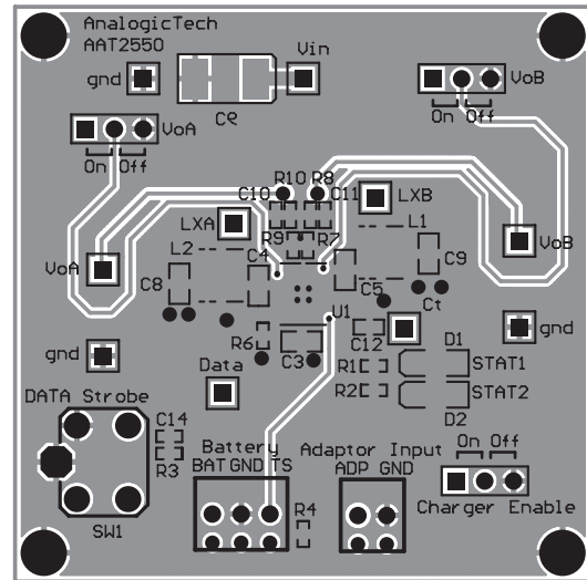
Figure 6: AAT2550 Evaluation Board Bottom Side Layout.
