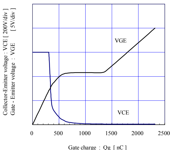
Dynamic Gate charge (typ.) Vcc=900V, Ic=450A, Tj= 25°C
