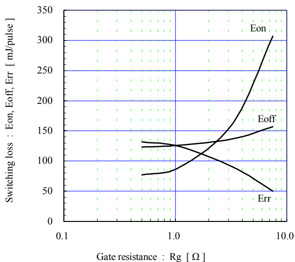
Switching loss vs. Gate resistance (typ.) V_{cc}=900V , I_c=450A , V_{GE}=\pm 15V , T_j=125^\circ C
