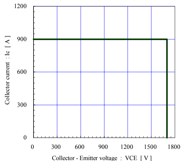
Reverse bias safe operating area (max.) +V_{GE}=15V , -V_{GE}\leq 15V , R_g\geq 1.1\Omega , T_j\leq 125^\circ C Stray inductance \leq 100nH
