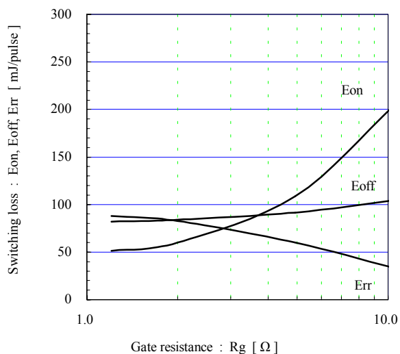
Switching loss vs. Gate resistance (typ.) V_{cc}=900V , I_c=300A , V_{GE}=\pm 15V , T_j=125^\circ C
