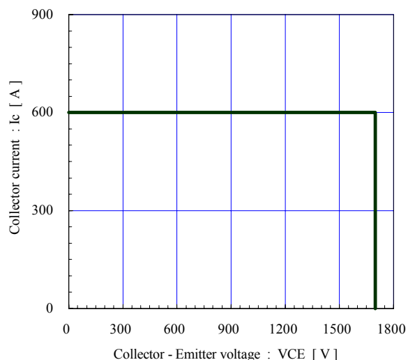
Reverse bias safe operating area (max.) +V_{GE}=15V , -V_{GE}\leq 15V , R_g\geq 2\Omega , T_j\leq 125^\circ C Stray inductance \leq 100nH
