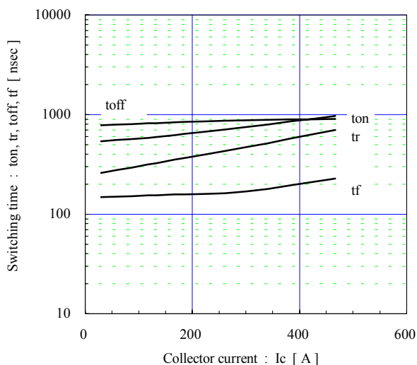
Switching time vs. Collector current (typ.) V_{cc}=900V , V_{GE}=\pm 15V , R_g=2\Omega , T_j=125^\circ C
