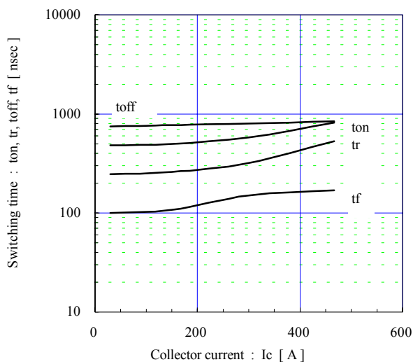
Switching time vs. Collector current (typ.) V_{cc}=900V , V_{GE}=\pm 15V , R_g=2\Omega , T_j=25^\circ C
