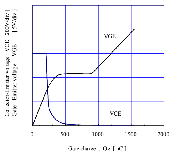
Dynamic Gate charge (typ.) V CC = 900V, Ic = 300A, T j = 25°C
