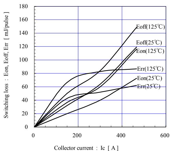
Switching loss vs. Collector current (typ.) V_{cc}=900V , V_{GE}=\pm 15V , R_g=2\Omega
