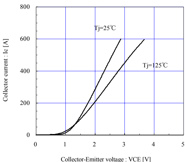
Collector current vs. Collector-Emitter voltage (typ.) VGE = 15V (typ.) / chip
