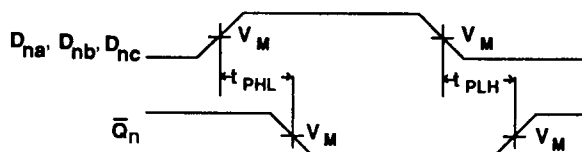
Waveform 1. For Inverting Outputs ('F10)
