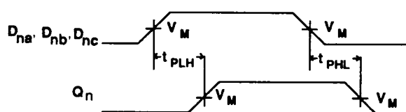
Waveform 2. For Non-Inverting Outputs ('F11)
