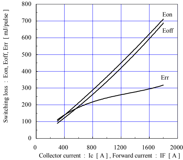
Switching loss vs. Collector current (typ.) V_{cc}=900V, V_{GE}=\pm 15V, R_{gon}=0.1\Omega, R_{goff}=0.4\Omega, T_j=125^\circ C
