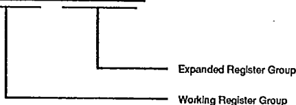
Figure 8. Register Pointer Register
