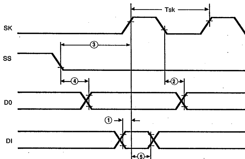
Figure 15. SPI Timing
