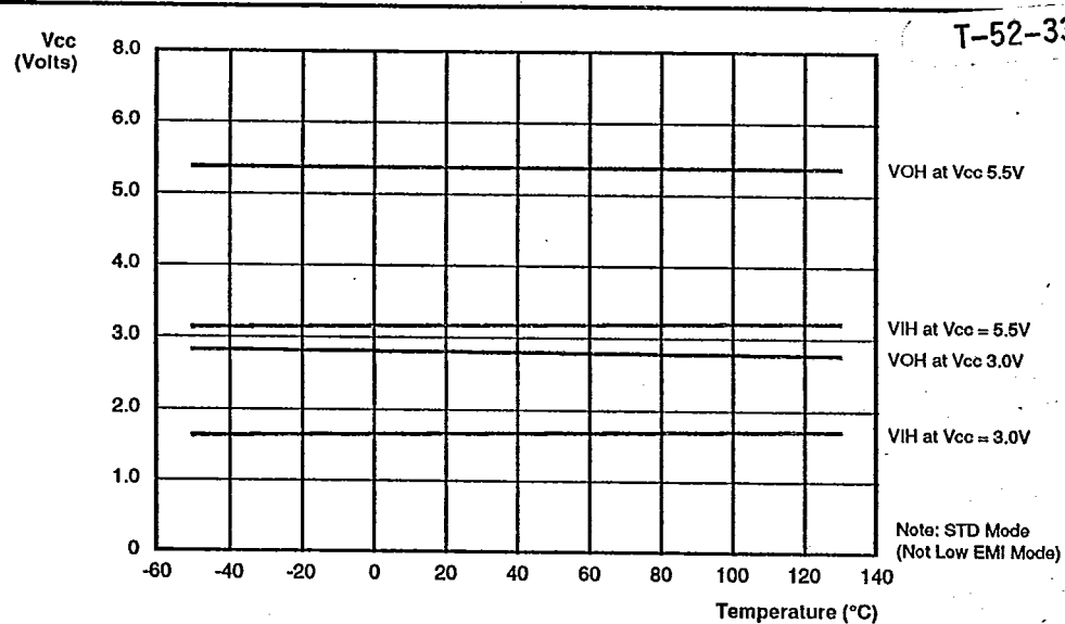
Figure 46. Typical V_{OH} , V_{IH} vs Temperature
