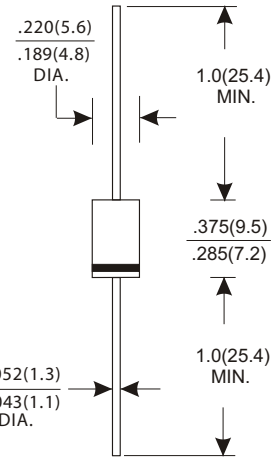
DO-27
