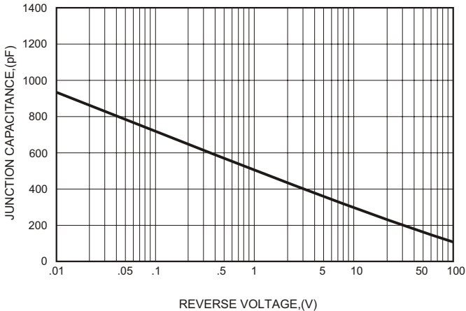
FIG.4-TYPICAL JUNCTION CAPACITANCE
