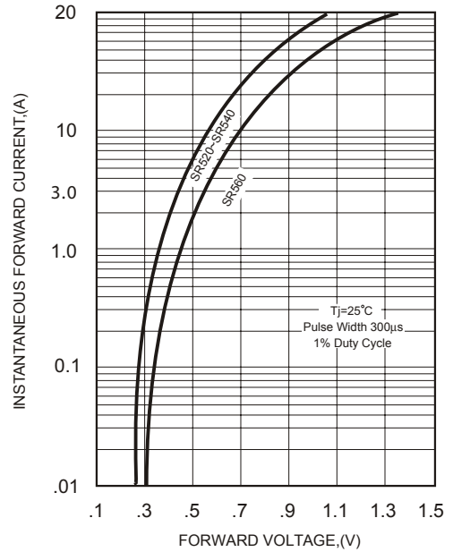
FIG.2-TYPICAL FORWARD CHARACTERISTICS
