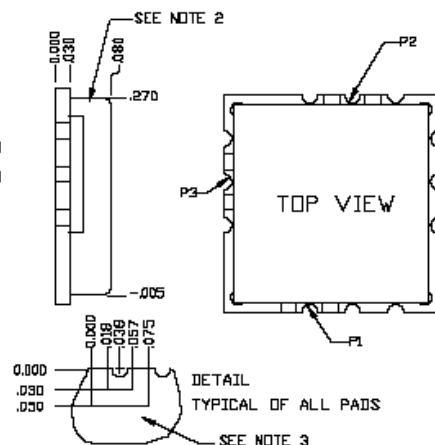
PHYSICAL DIMENSIONS
