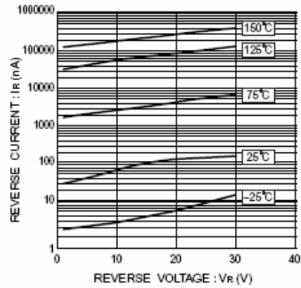
Fig.2 Reverse characteristics
