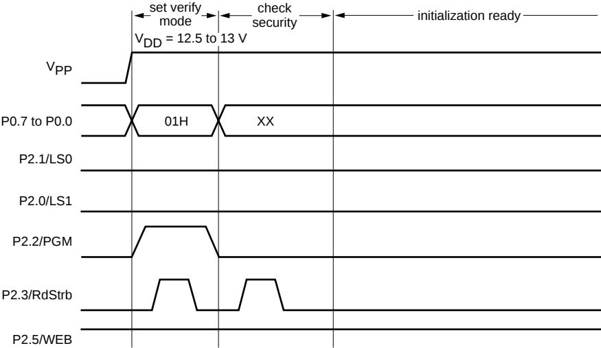
Fig.71 Parallel program mode initialization.
