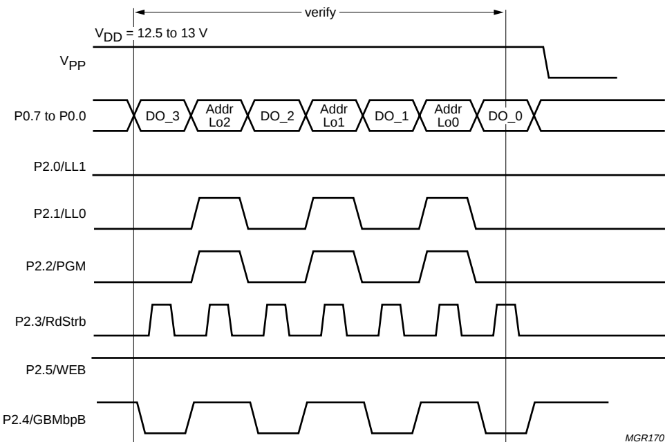
Fig.74 Multiple byte programming mode (verify).
