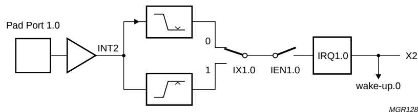
Fig.32 Interrupt Port 1.0.
