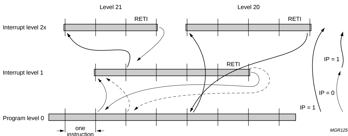
Fig.29 Interrupt hierarchy.
