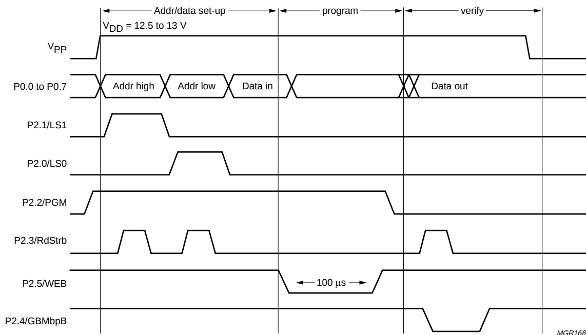
Fig.72 Single byte programming mode.
