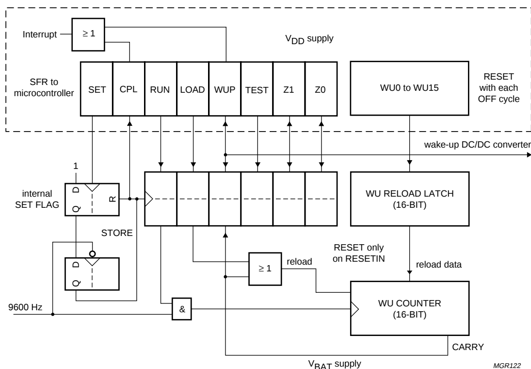
Fig.21 Block diagram of wake-up counter.
