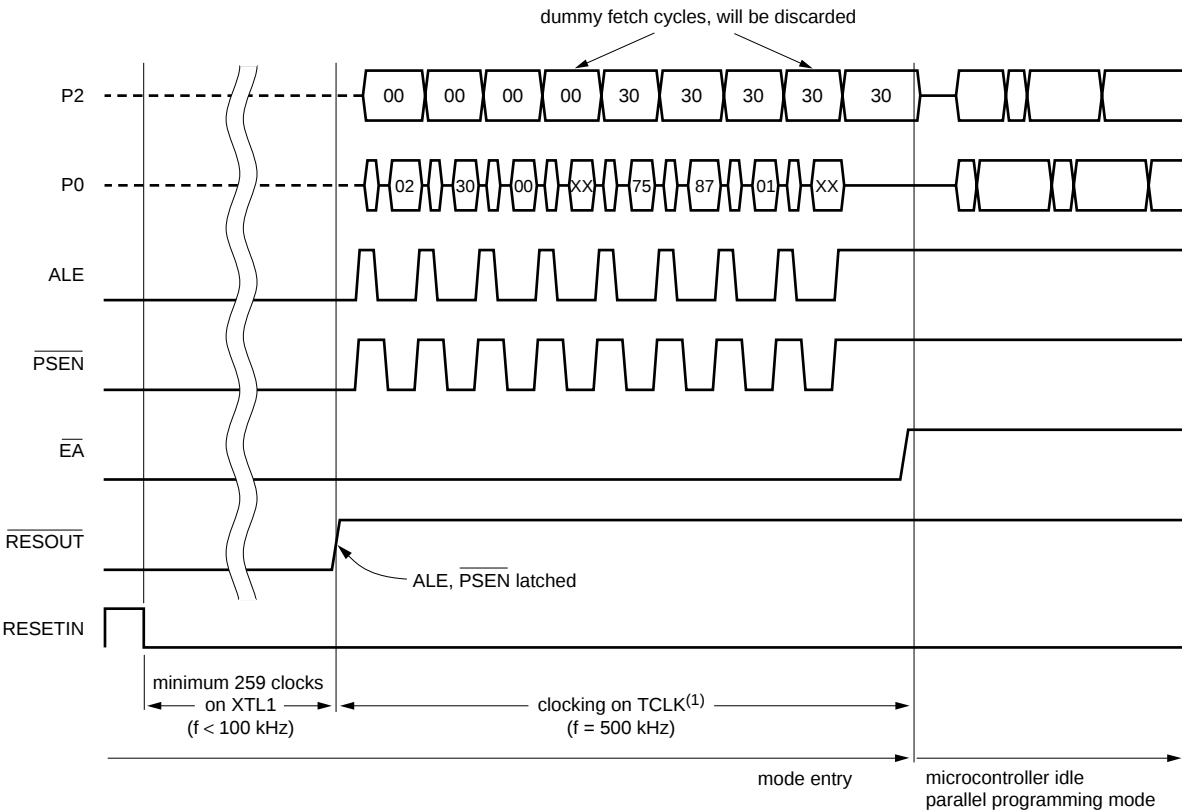
Fig.70 Program mode entry.
