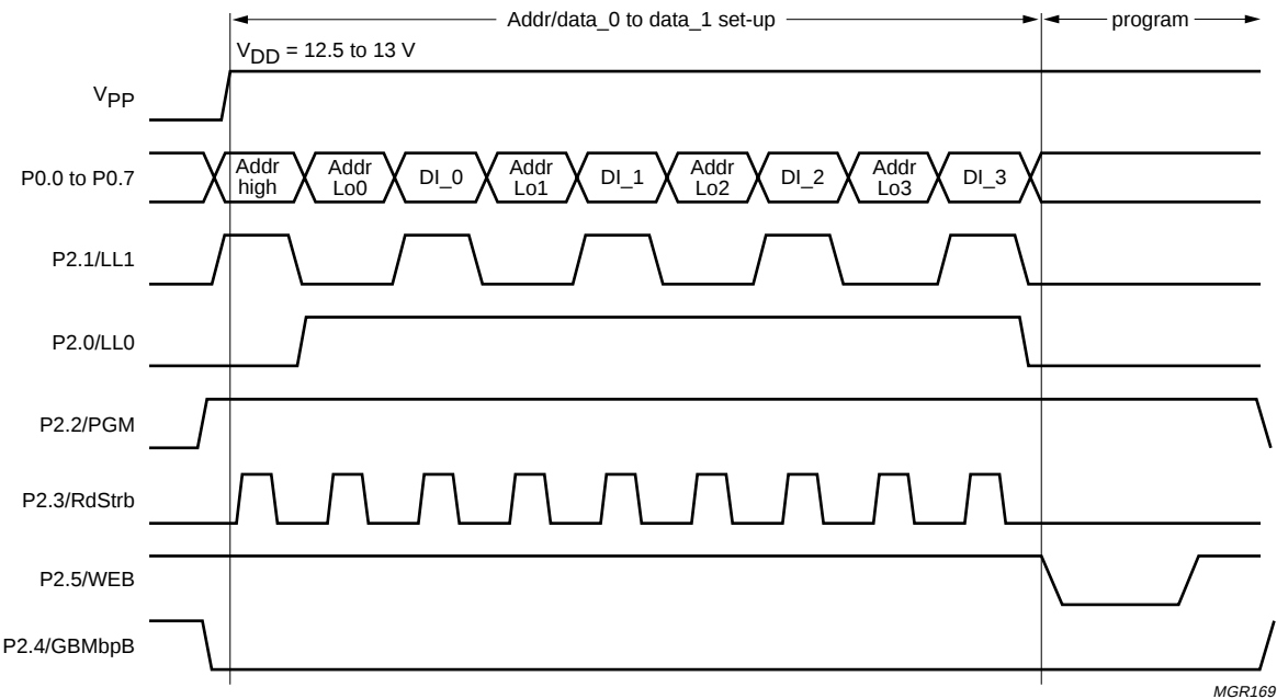
Fig.73 Multiple byte programming mode (address and data load, programming pulse).
