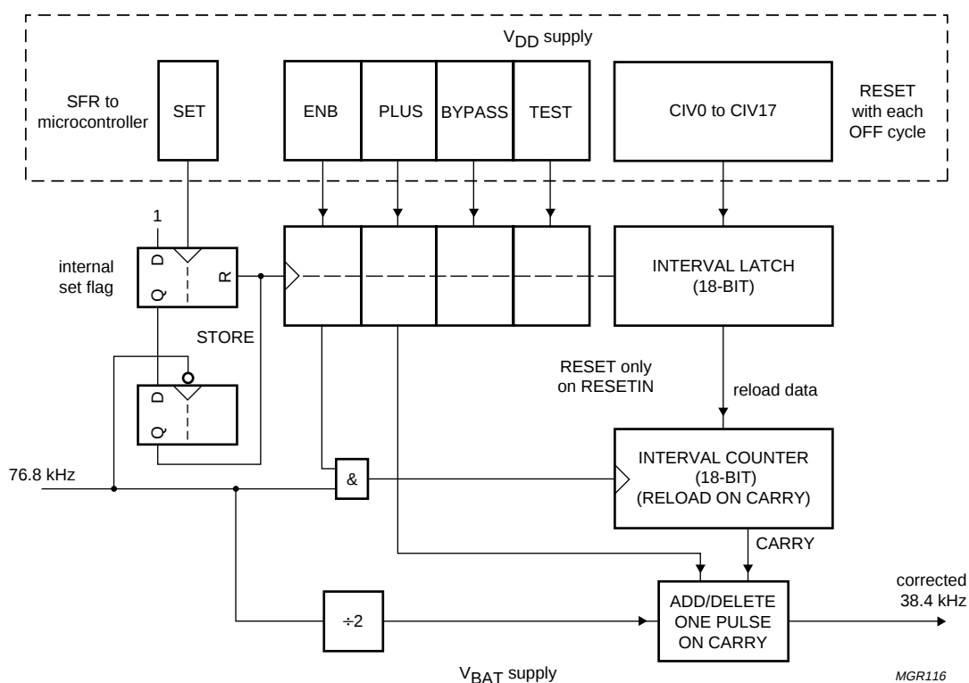
Fig.15 Block diagram of clock compensation.
