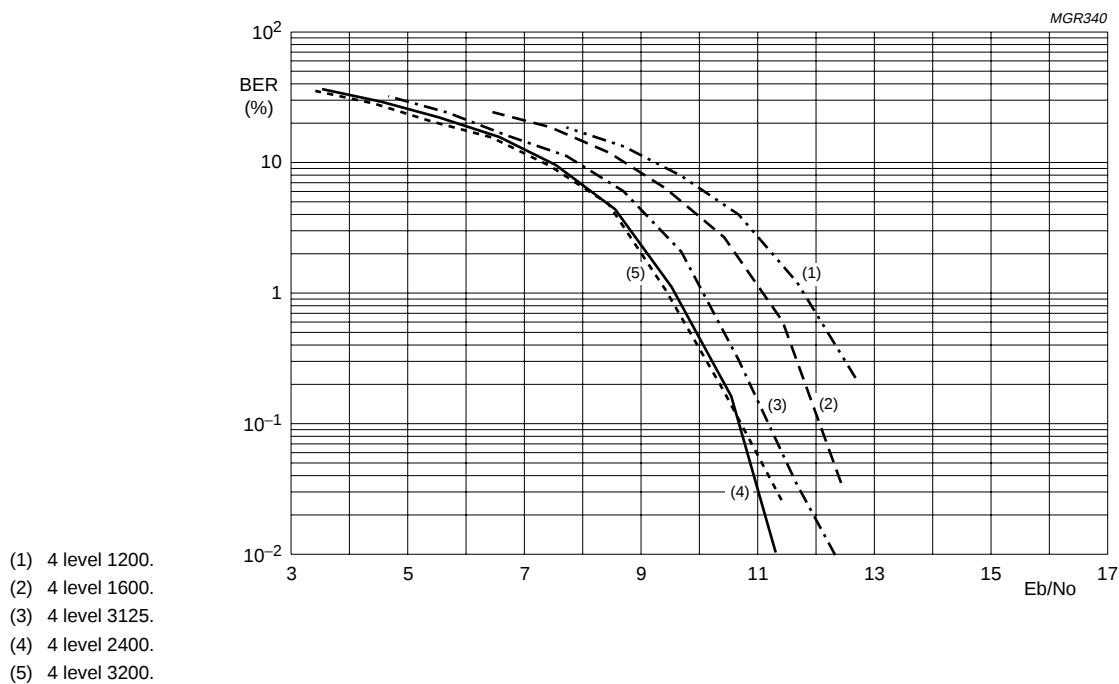
Fig.25 Demodulator performance in 4L mode.
