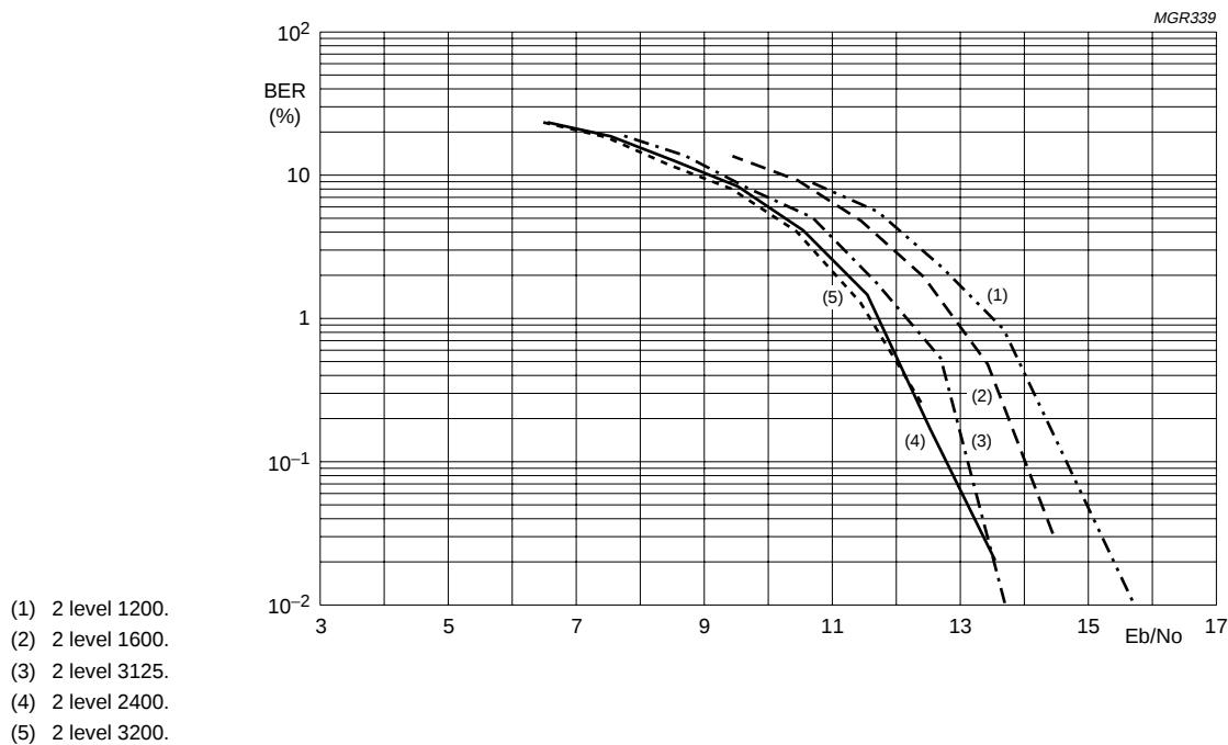
Fig.24 Demodulator performance in 2L mode.
