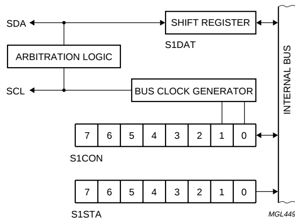
Fig.8 Block diagram of I 2 C-bus serial I/O.
