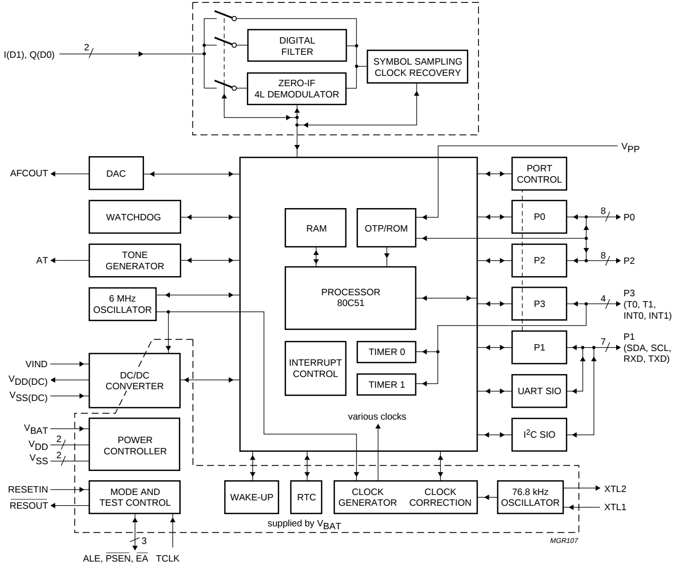
Fig.1 Block diagram.
