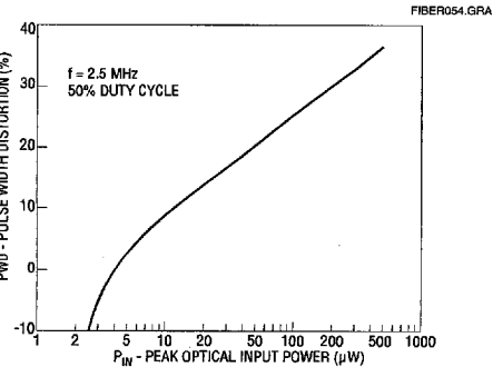
Fig. 1 Pulse Width Distortion vs Optical Input Power
