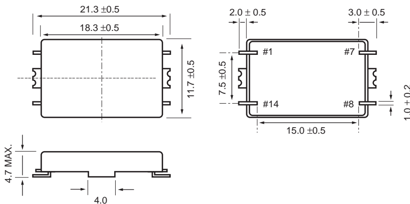
ECS-TXO-10C2 SERIES – Top, Side and Bottom views
