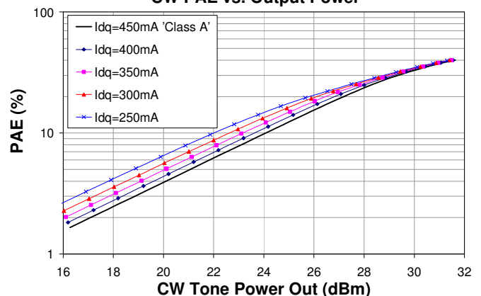
CW PAE vs. Output Power
