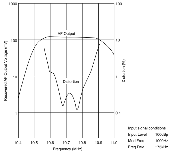
Frequency Characteristics
