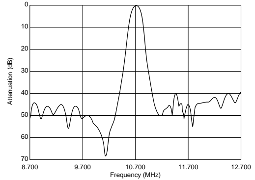
SFELA10M7HAA0-B0
