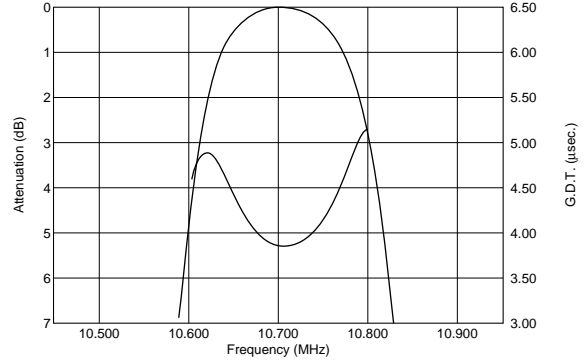
SFELA10M7HAA0-B0
