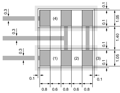
(1) : Input (2) : Ground (3) : Float Signal Line (4) : Out put [Shaded Box] It shows solder resist land pattern.
