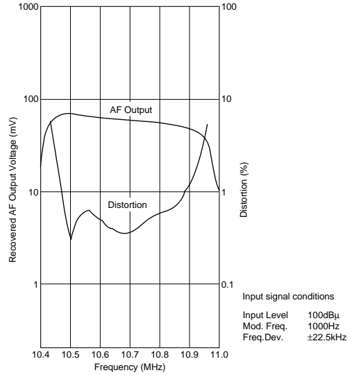
Frequency Characteristics
