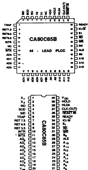
Figure 2 : PDIP and PLCC PIN CONFIGURATIONS
