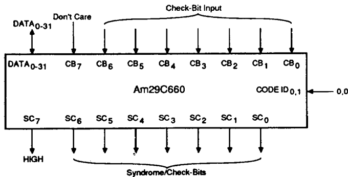
Figure 2. 32-Bit Configuration
