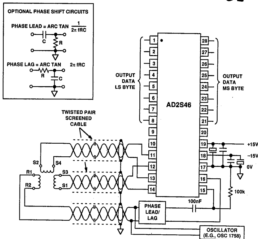
Figure 1. Connection Diagram
