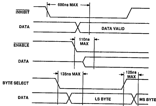
Figure 2. Timing Diagrams
