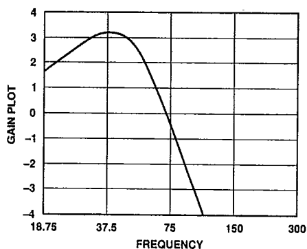
Figure 3. AD2S46 Gain Plot
