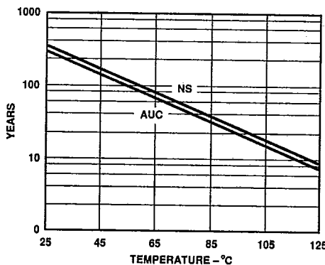
Figure 5. AD2S46 MTBF vs. Temperature
