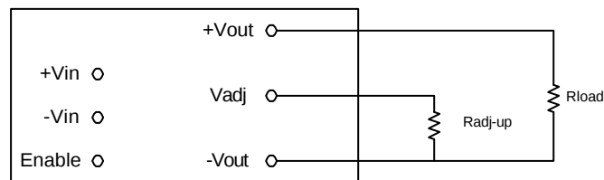
Figure 15 . Circuit Configuration to Increase Output Voltage.
