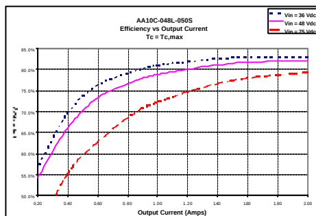
Figure 5. 050S Efficiency vs Load Current.
