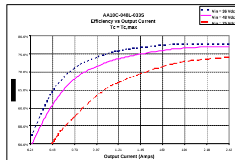
Figure 4. 033S Efficiency vs Load Current.
