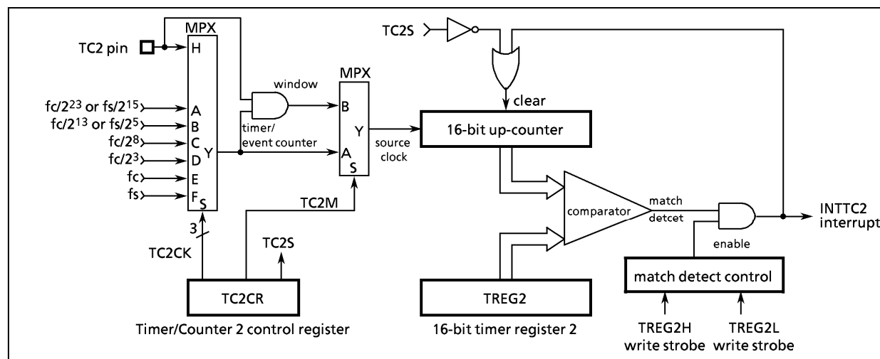
Figure 2-27. Timer/Counter 2 (TC2)
