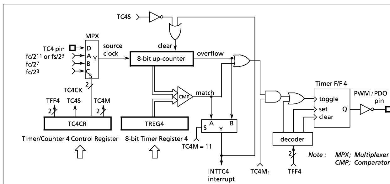
Figure 2-34. Timer/Counter 4
