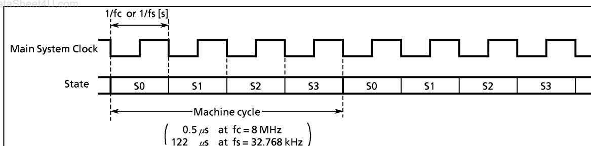
Figure 1-13. Machine Cycle
