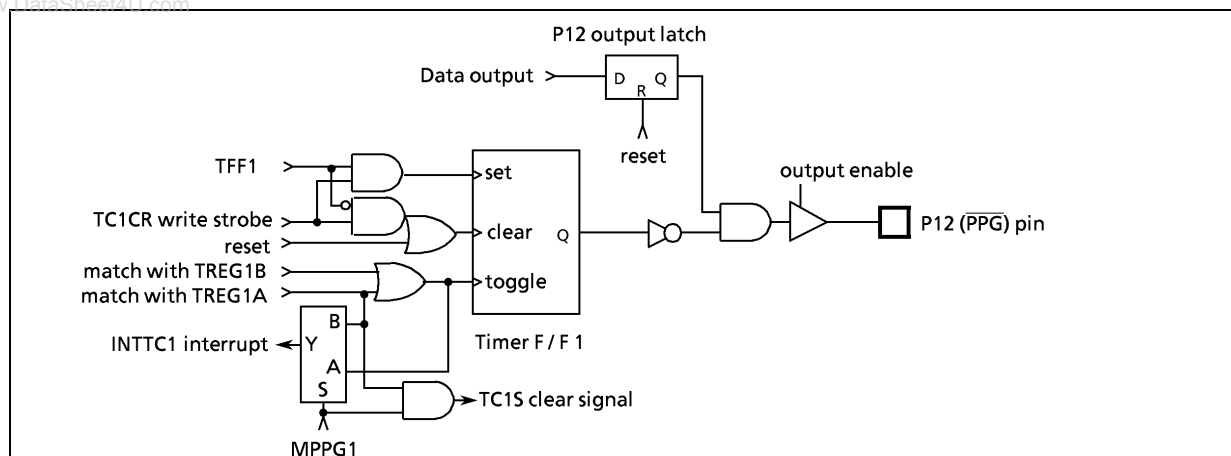
Figure 2-26. PPG Output
