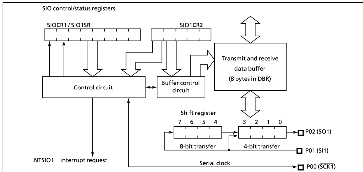
Figure 2-63. Serial Interfaces
