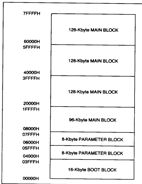
Figure 10. 28F004BX-BL Memory Map
