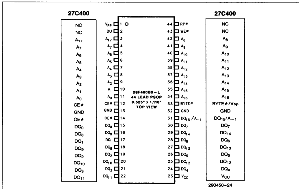
Figure 3. PSOP Lead Configuration for x8/x16 28F400BX-L
