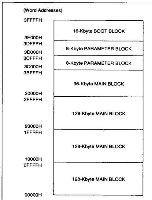
Figure 8. 28F400BX-TL Memory Map
