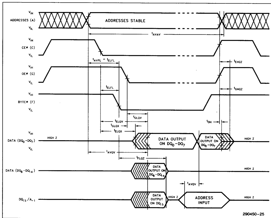
Figure 17. BYTE # Timing Diagram for Both Read and Write Operations for 28F400BX-L
