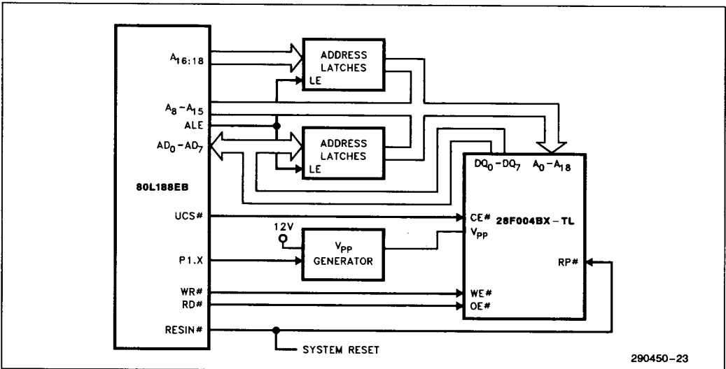
Figure 2. 28F004BX-L interface to INTEL 80L188EB Low Voltage 8-bit Embedded Microprocessor
