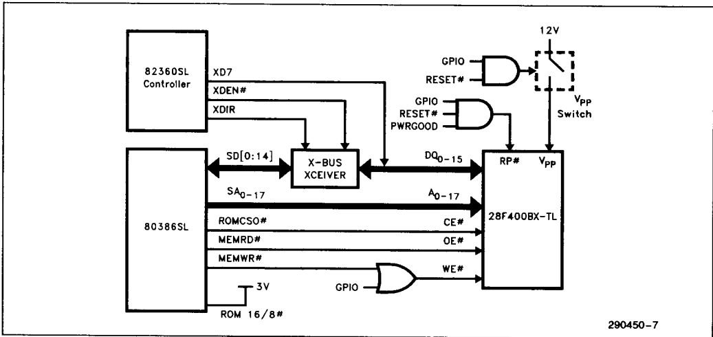
Figure 1. 28F400BX-L interface to INTEL386SL 3.3V Microprocessor Superset
