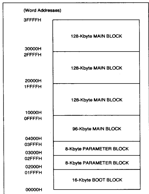
Figure 7. 28F400BX-BL Memory Map
