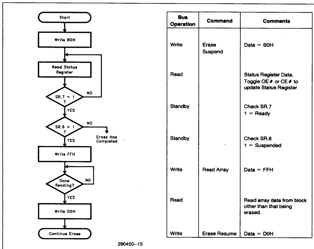
Figure 15. Erase Suspend/Resume Flowchart
