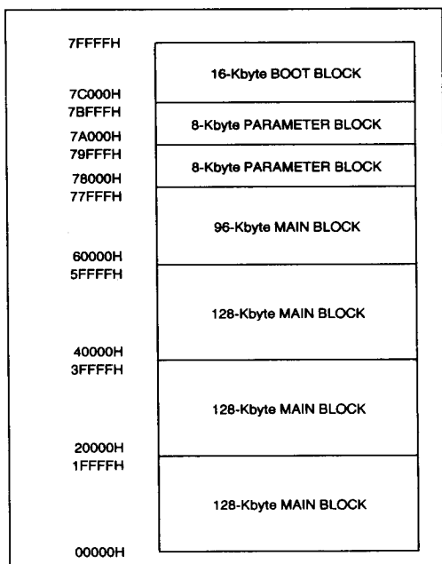
Figure 11. 28F004BX-TL Memory Map
