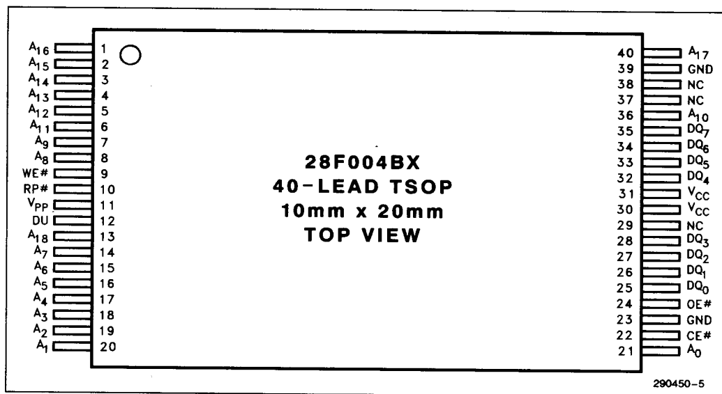
Figure 5. TSOP Lead Configuration for x8 28F004BX-L
