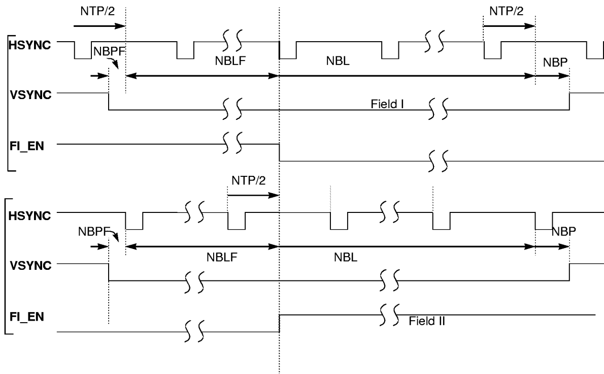
Figure 19. Field Index: (short HSYNC, long VSYNC, width of NBL is non-integer number of lines) Note: Sync. signals are always outputs for the short HSYNC, long VSYNC case.
