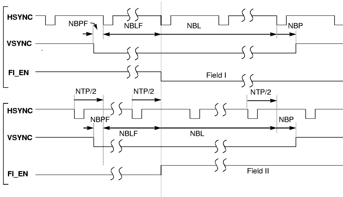
Figure 18. Field Index: (short HSYNC, long VSYNC, width of NBL is integer number of lines) Note: Sync. signals are always output for the short HSYNC, long VSYNC case
