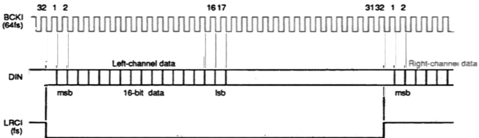
Figure 4. Input timing ( \overline{IW18} = \text{HIGH or open} )
