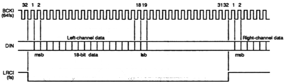
Figure 3. Input timing ( \overline{IW18} = \text{LOW} )
