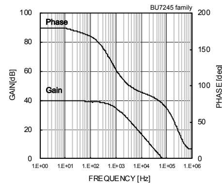
Fig. 92 Gain – Frequency
