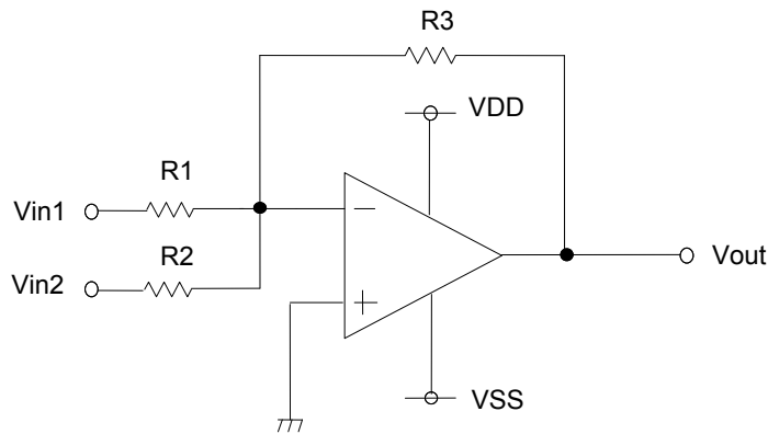
Fig.170 Adder circuit
