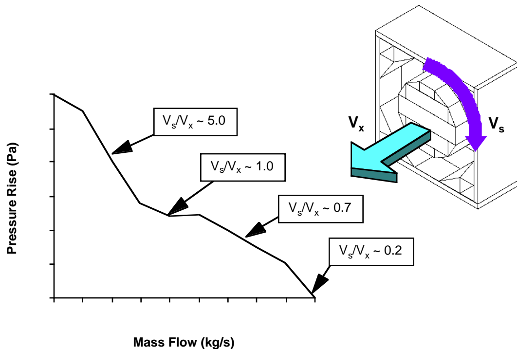
Figure C.1 - Representative Values of Swirl Coefficient V_s/V_x [HARMESEN,2]
