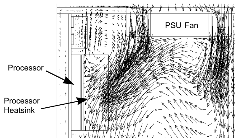
Figure 11 - Results for the Fan Blowing Configuration Close-up of Flows Through the Processor Heatsink
