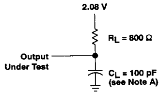
Figure 2. AC Test Output Load Circuit
