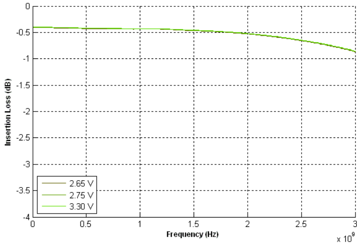
Figure 6. Insertion Loss: RFC-RF @ 25 °C
