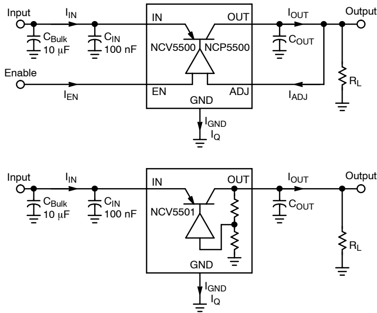
Figure 3. Measuring Circuits
