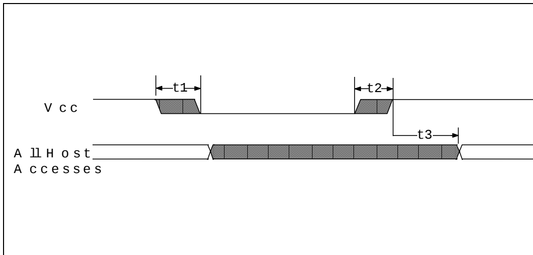
FIGURE 6 - POWER-UP TIMING
