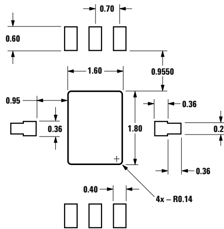
Figure 26. Stencil outline drawing (mm).
