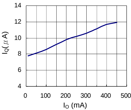
Quiescent Current vs. Load
