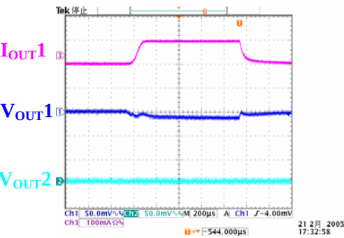
Load Transient Regulation
