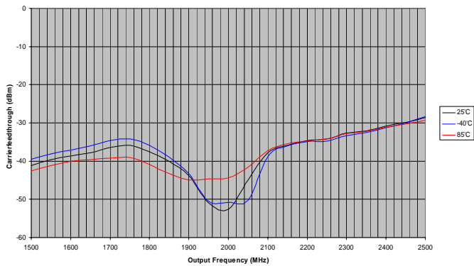
Figure 16. ADL5372 Uncalibrated Carrier Feed through
