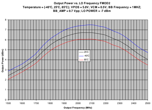
Figure 6. ADL5372 Output Power vs. Frequency and Temperature. Baseband drive is 1.4 Vpp differential
