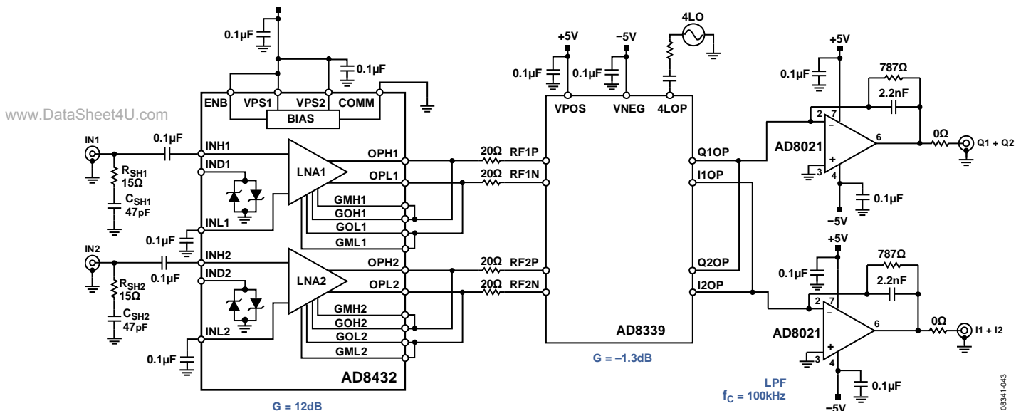
Figure 66. Schematic of AD8432 (G = 12.04 dB) + AD8339 Application for Ultrasound Beamforming
