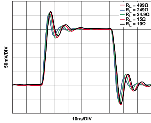
Figure 38. Small Signal Transient Response vs. Resistive Load ( R_L ), G = 12.04 dB
