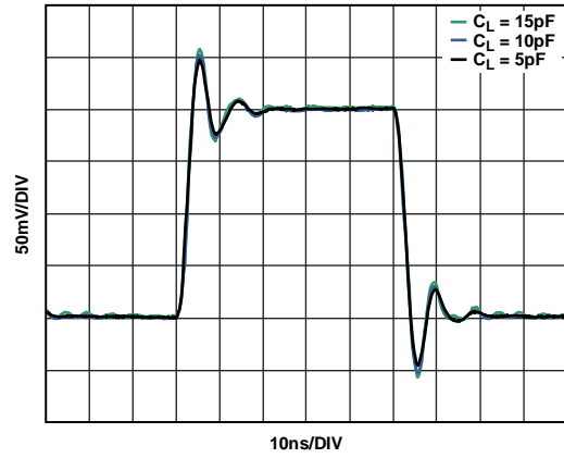
Figure 36. Small Signal Transient Response vs. Capacitive Load ( C_L ), G = 12.04 dB
