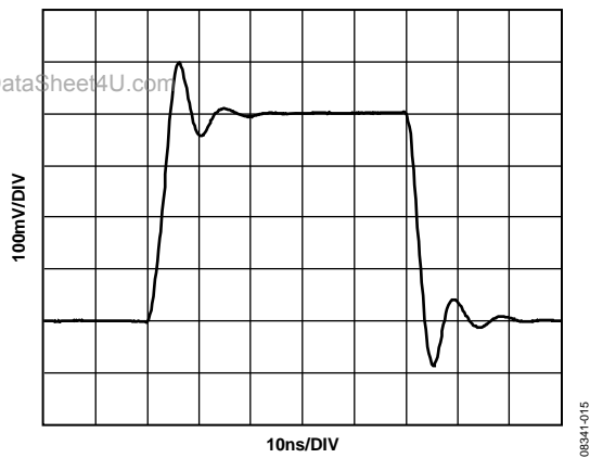
Figure 35. Small Signal Transient Response, G = 12.04 dB
