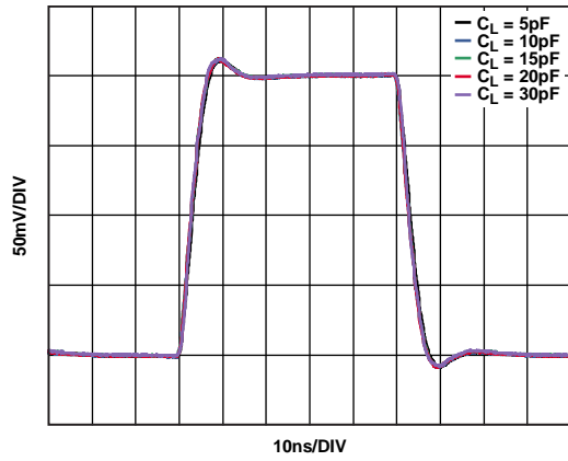
Figure 37. Small Signal Transient Response vs. Capacitive Load ( C_L ), G = 24.08 dB
