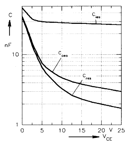
Fig. 8 Typ. capacitances
