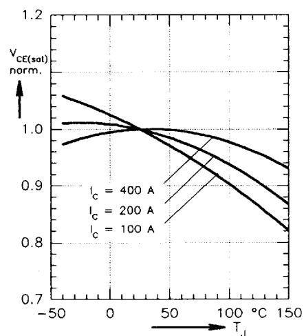
Fig. 4 Typ. temperature dependence of normalized V_{CE(sat)}
