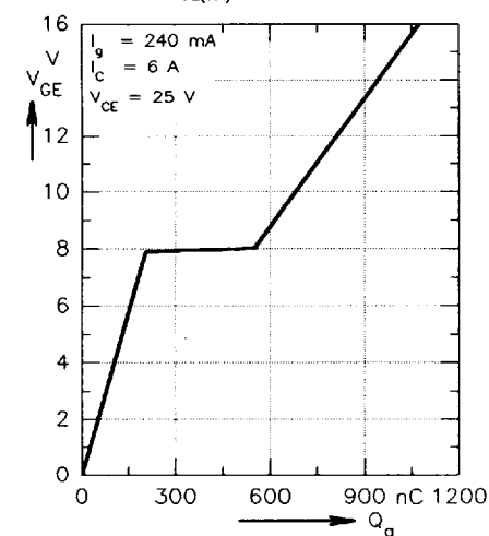
Fig. 7 Typ. turn-on gate charge characteristics
