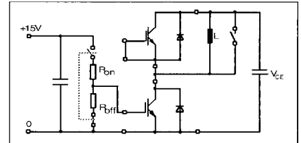
Test circuit for E_{on} , E_{off} , SCSOA and RBSOA R_{on} = 1.2 \Omega , L = 100 \mu\text{H} R_{off} = 3.6 \Omega for RBSOA, E_{off}
