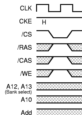
Fig.9 No operation
