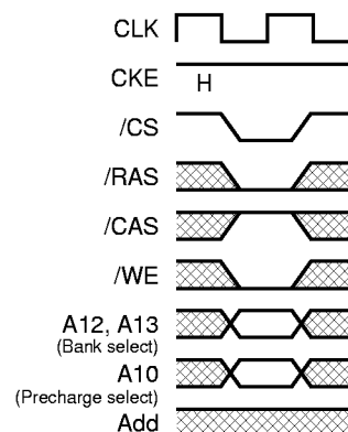
Fig.3 Precharge command
